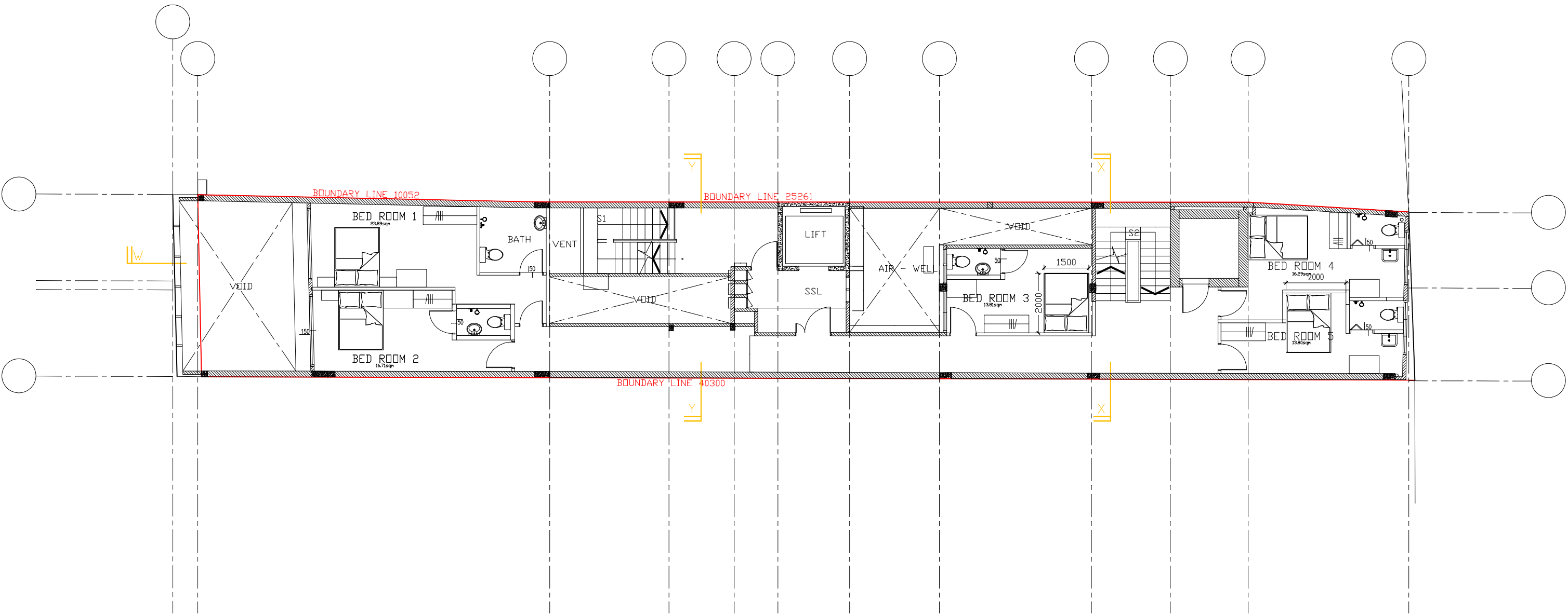
4TH STOREY PLAN
